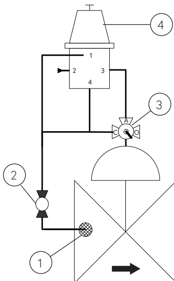
Pressure Sustaining
