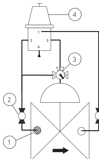
Pressure Reducing
